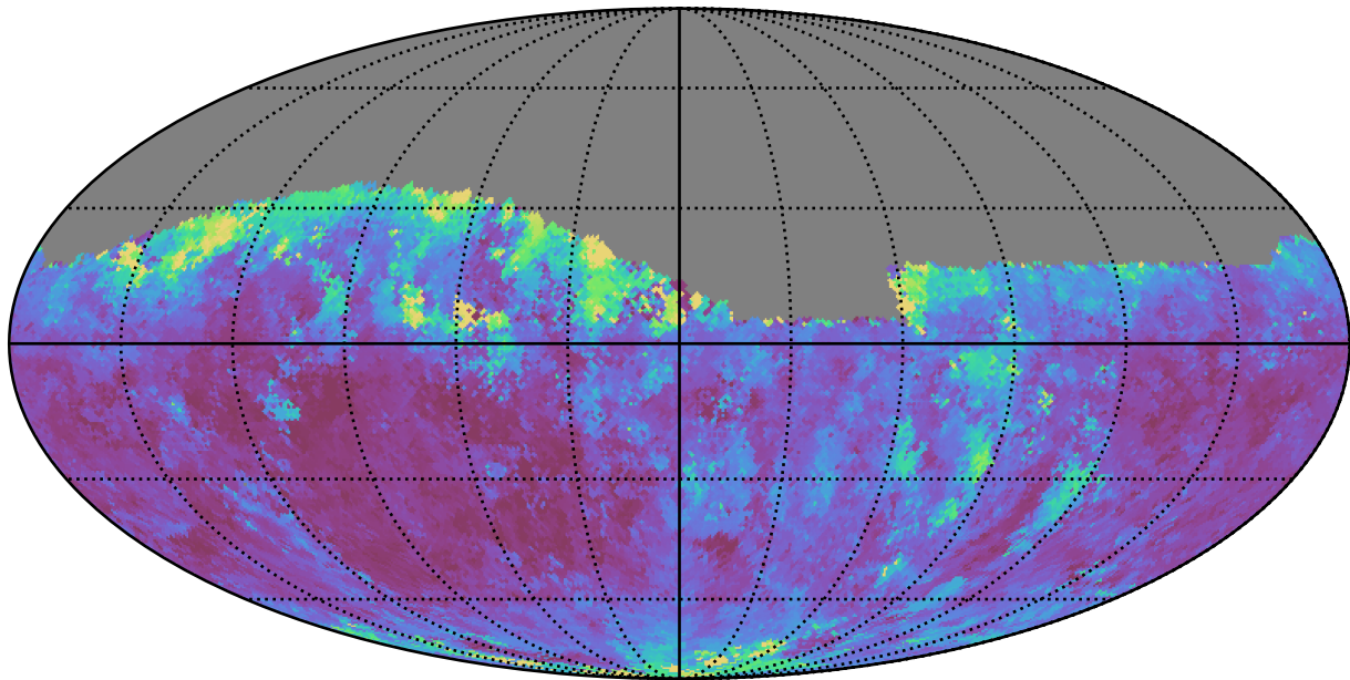
roll_pause_mjdp365_v3.4_10yrs Yr 1 z band: Median seeingEff
