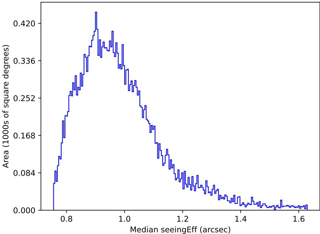
roll_pause_mjdp365_v3.4_10yrs Yr 1 z band: Median seeingEff
