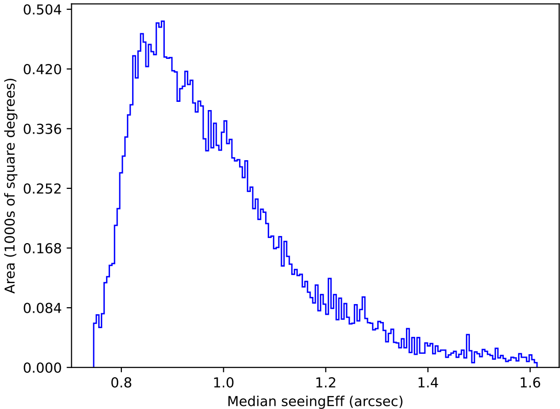
roll_pause_mjdp365_v3.4_10yrs Yr 1 r band: Median seeingEff
