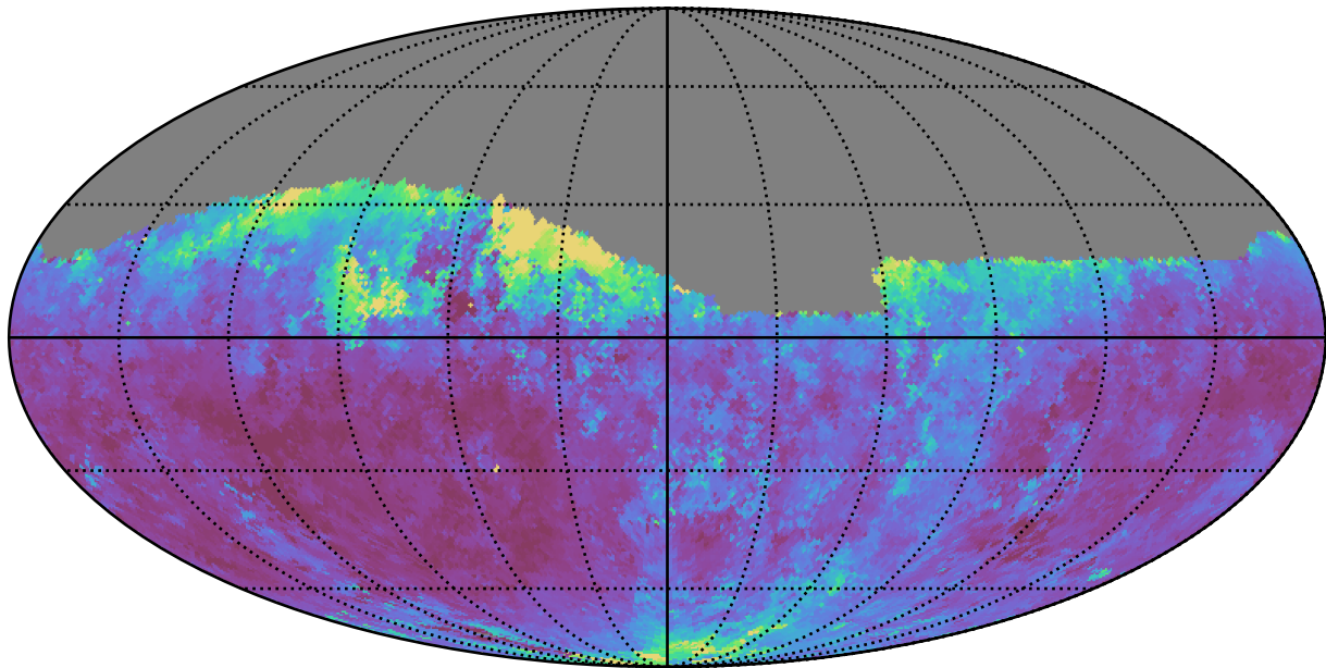
roll_pause_mjdp365_v3.4_10yrs Yr 1 i band: Median seeingEff
