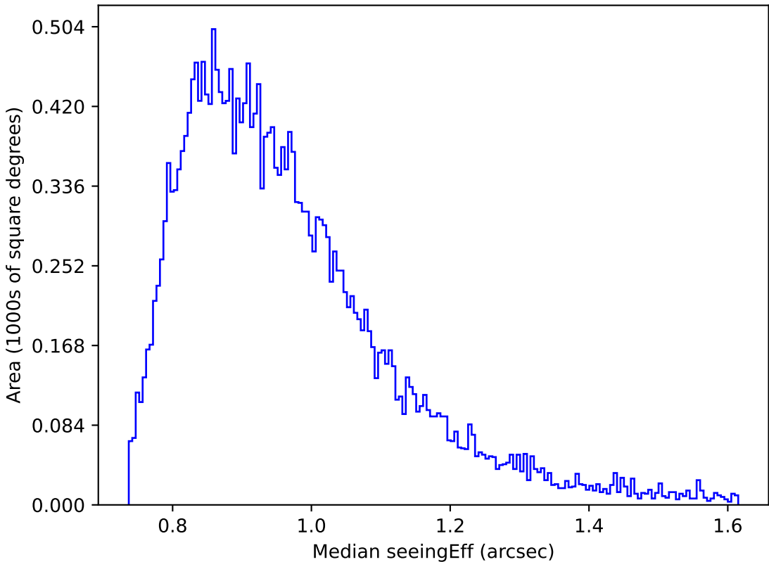
roll_pause_mjdp365_v3.4_10yrs Yr 1 i band: Median seeingEff
