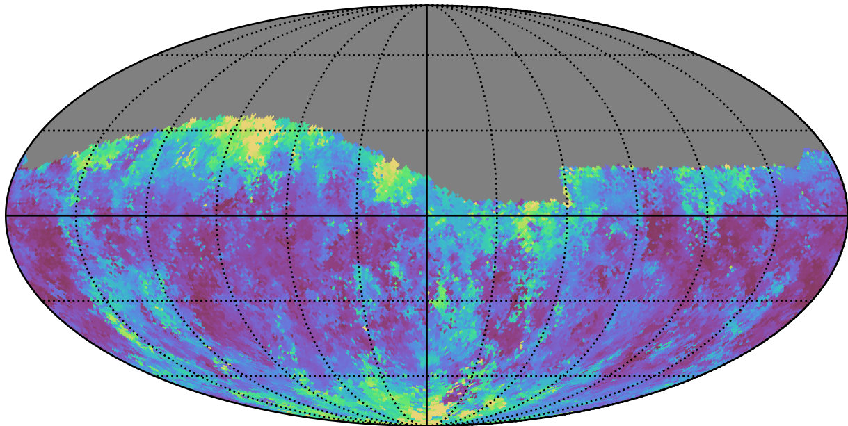
roll_pause_mjdp365_v3.4_10yrs Yr 1 g band: Median seeingEff
