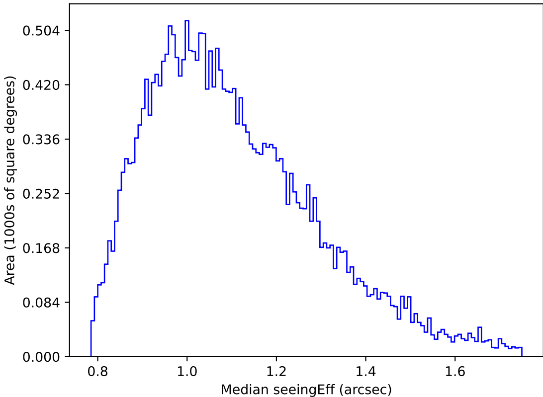
roll_pause_mjdp365_v3.4_10yrs Yr 1 g band: Median seeingEff
