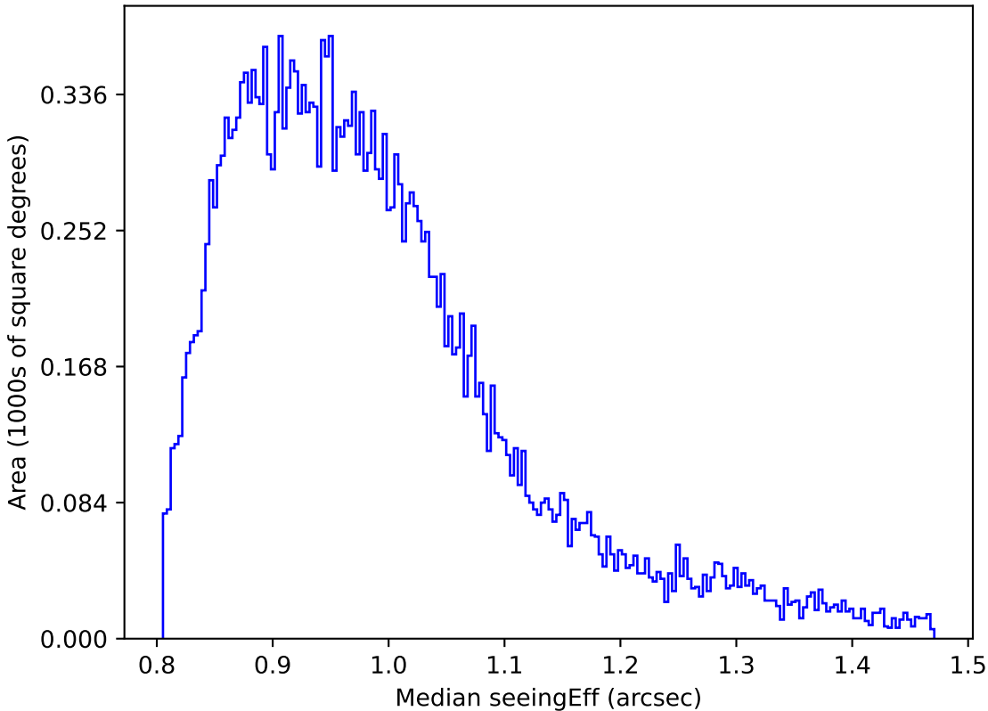
roll_pause_mjdp365_v3.4_10yrs Yr 1 all bands: Median seeingEff
