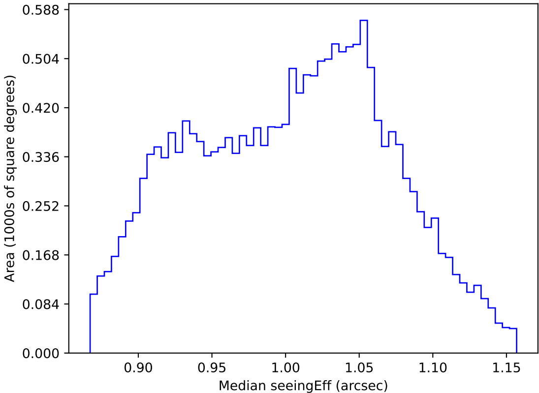
roll_pause_mjdp365_v3.4_10yrs WFD z band: Median seeingEff
