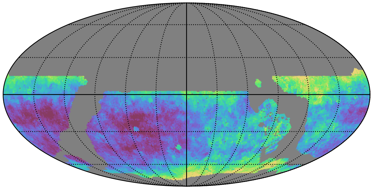
roll_pause_mjdp365_v3.4_10yrs WFD y band: Median seeingEff
