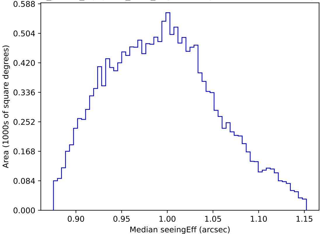
roll_pause_mjdp365_v3.4_10yrs WFD y band: Median seeingEff
