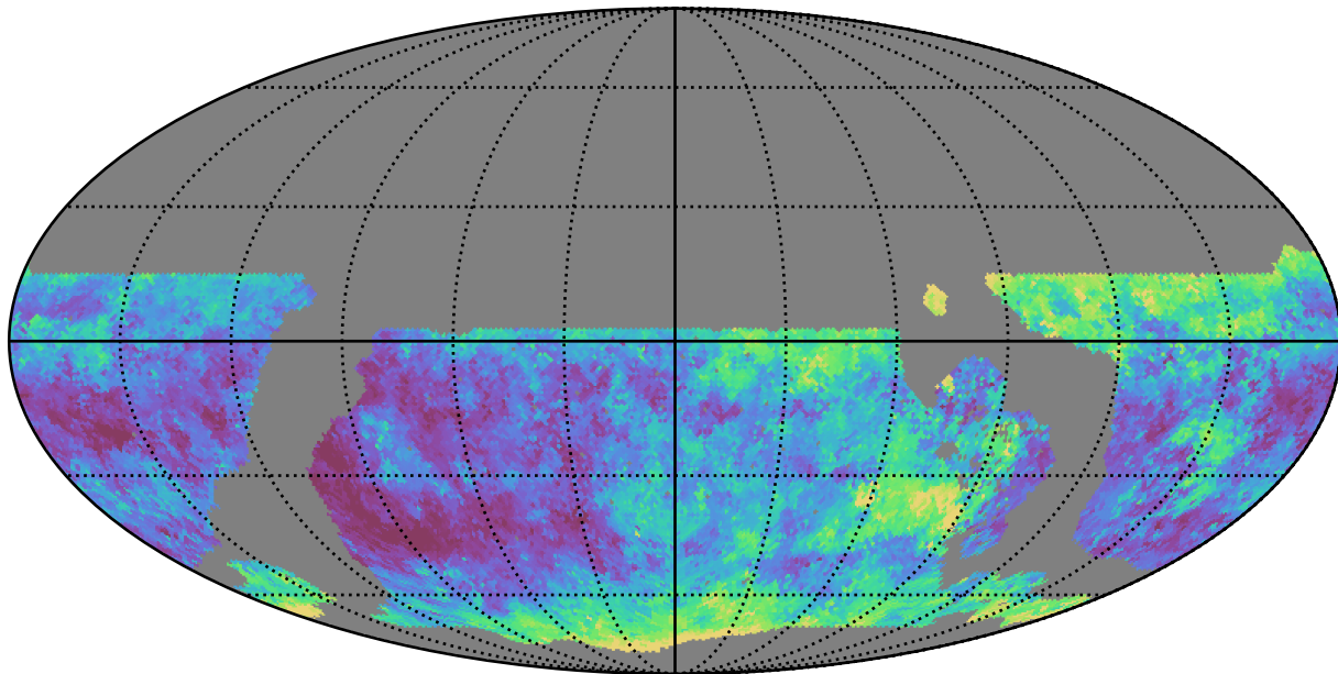
roll_pause_mjdp365_v3.4_10yrs WFD u band: Median seeingEff
