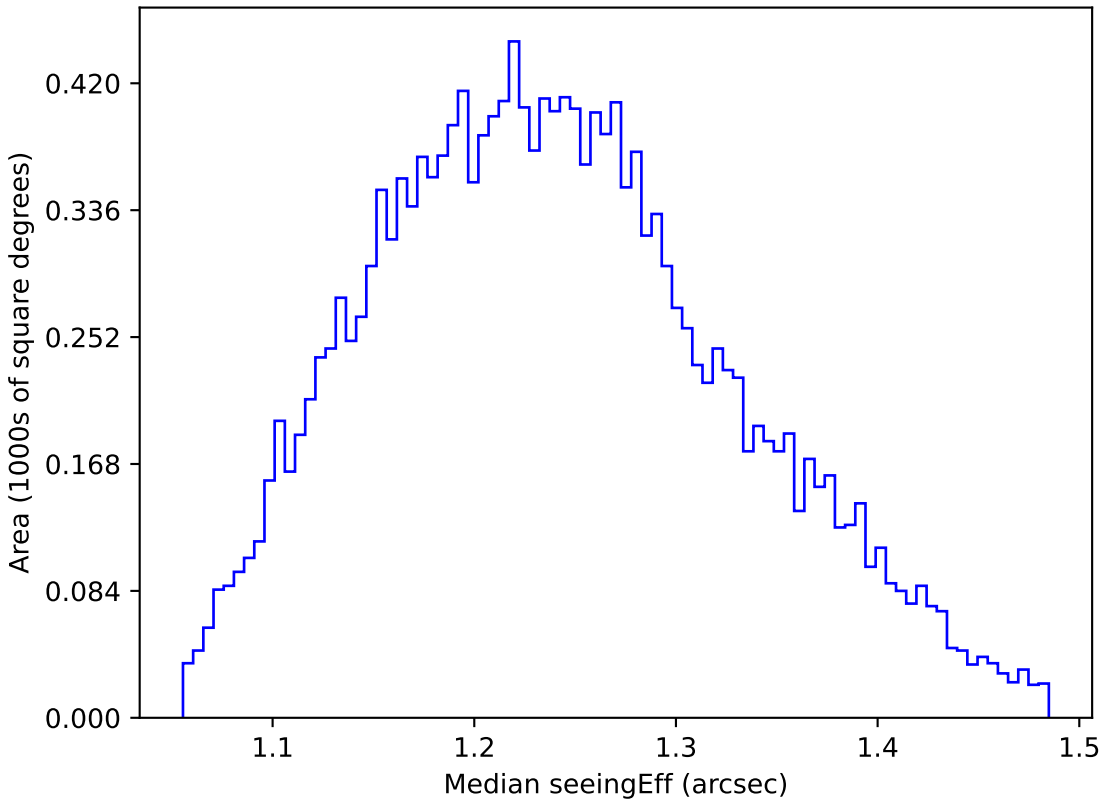
roll_pause_mjdp365_v3.4_10yrs WFD u band: Median seeingEff
