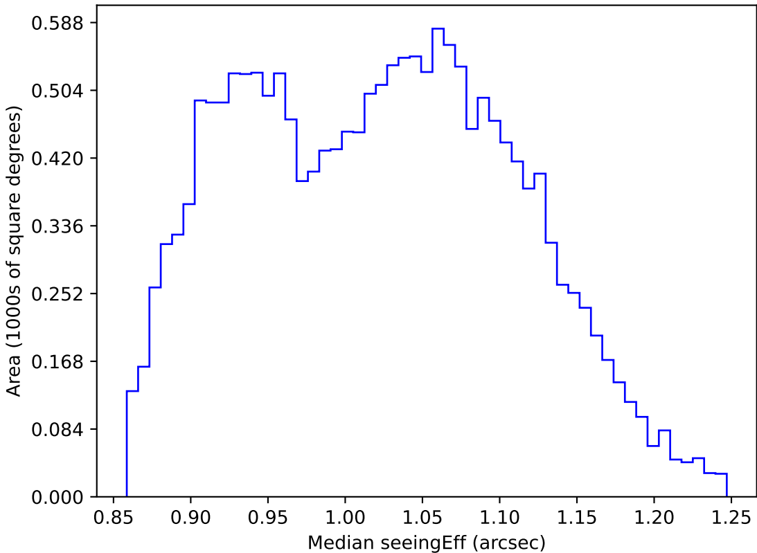
roll_pause_mjdp365_v3.4_10yrs WFD r band: Median seeingEff
