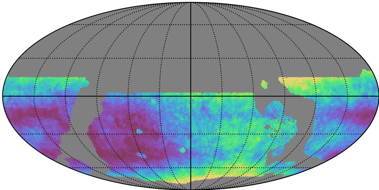
roll_pause_mjdp365_v3.4_10yrs WFD i band: Median seeingEff
