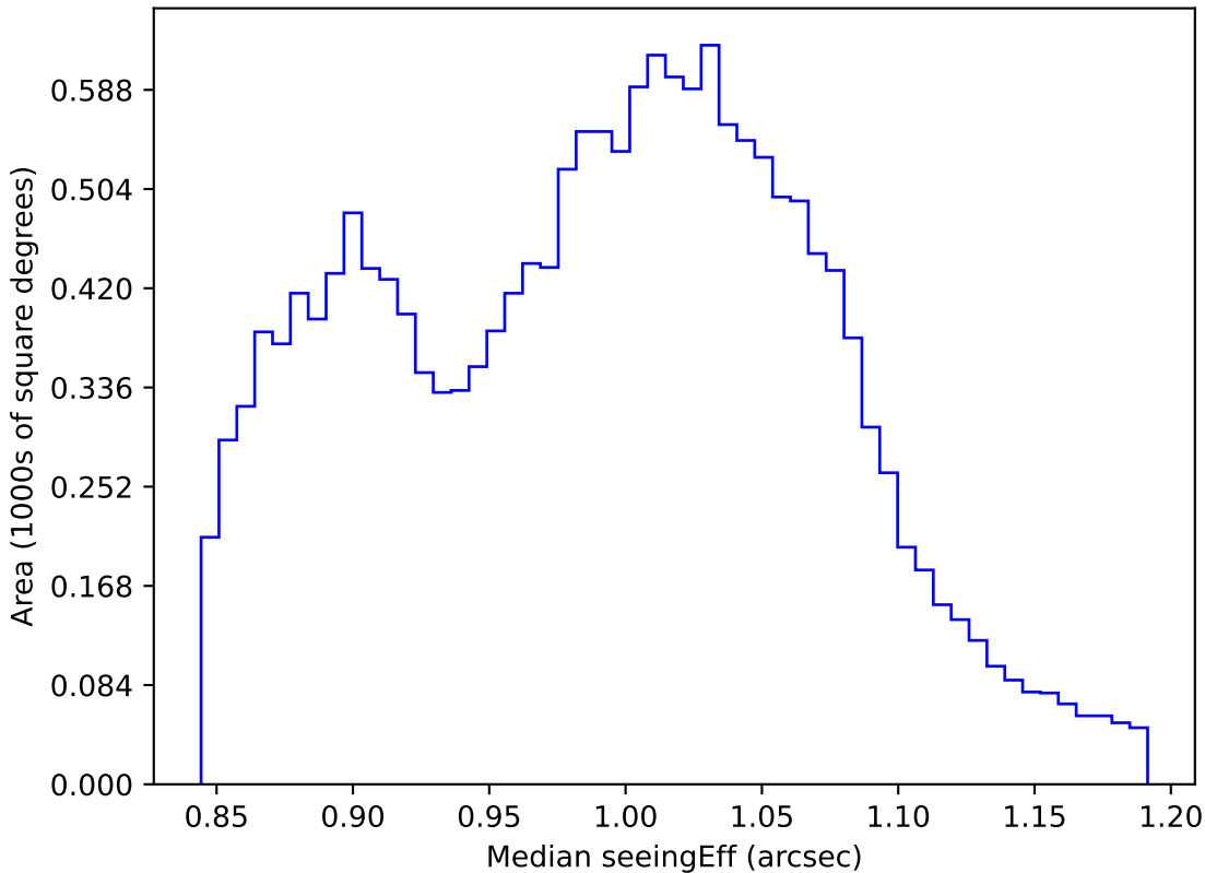
roll_pause_mjdp365_v3.4_10yrs WFD i band: Median seeingEff
