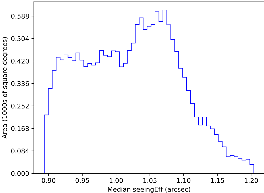
roll_pause_mjdp365_v3.4_10yrs WFD all bands: Median seeingEff
