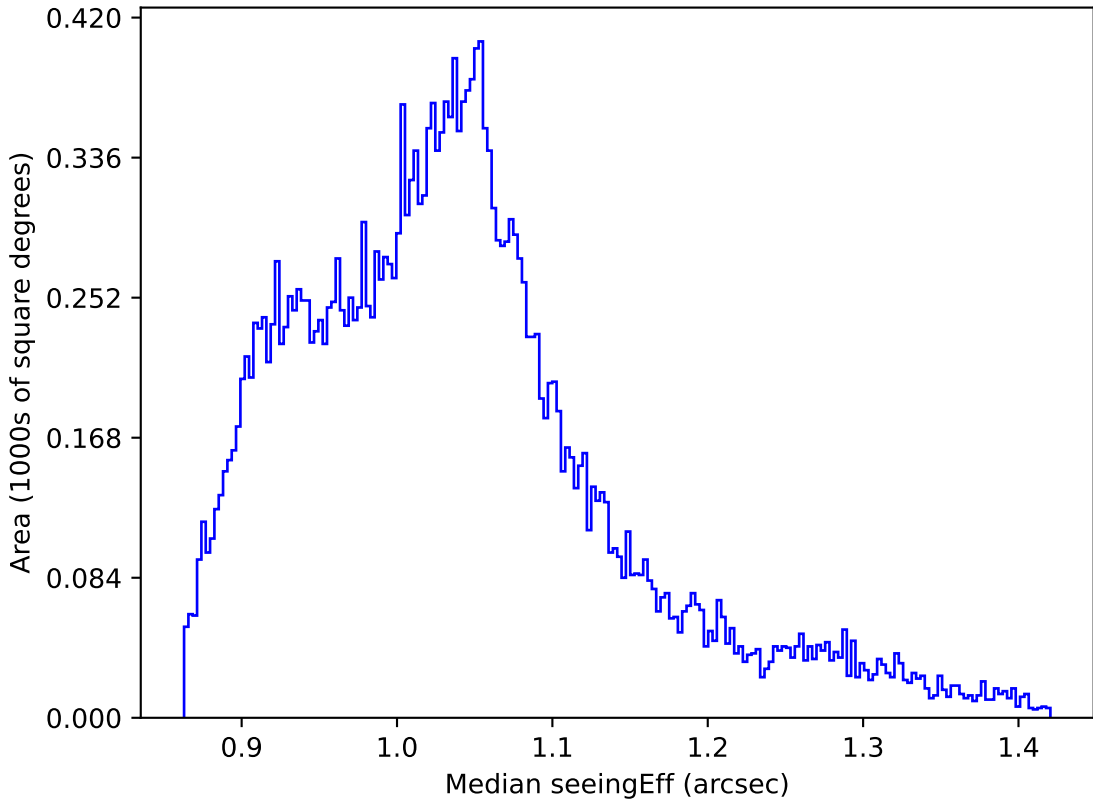
roll_pause_mjdp365_v3.4_10yrs All sky z band: Median seeingEff
