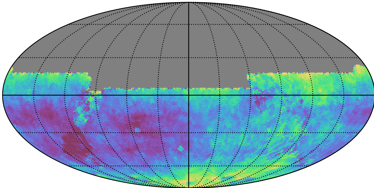
roll_pause_mjdp365_v3.4_10yrs All sky y band: Median seeingEff
