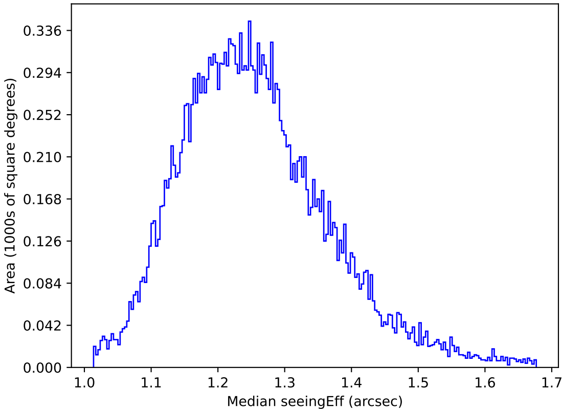
roll_pause_mjdp365_v3.4_10yrs All sky u band: Median seeingEff
