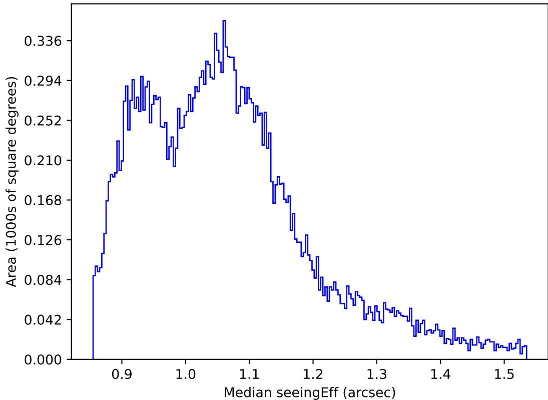
roll_pause_mjdp365_v3.4_10yrs All sky r band: Median seeingEff
