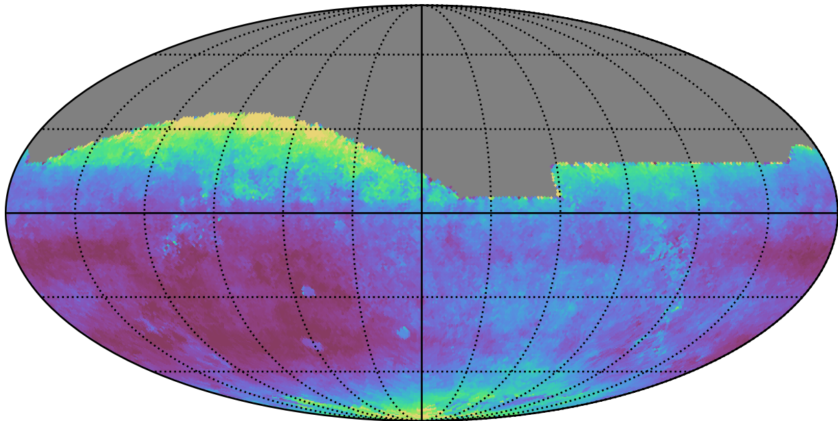
roll_pause_mjdp365_v3.4_10yrs All sky i band: Median seeingEff
