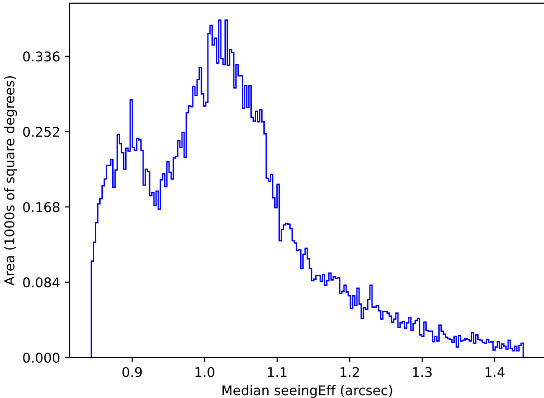
roll_pause_mjdp365_v3.4_10yrs All sky i band: Median seeingEff
