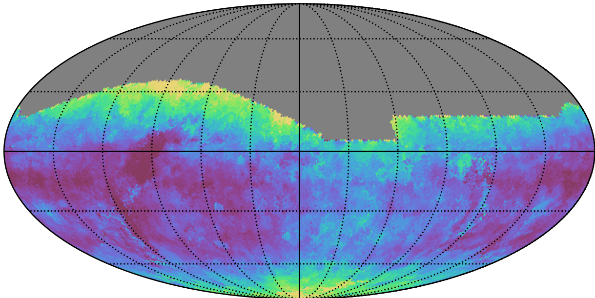
roll_pause_mjdp365_v3.4_10yrs All sky g band: Median seeingEff
