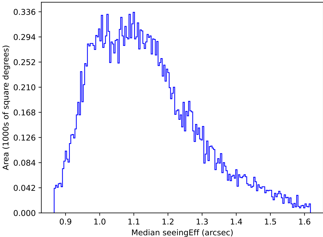
roll_pause_mjdp365_v3.4_10yrs All sky g band: Median seeingEff
