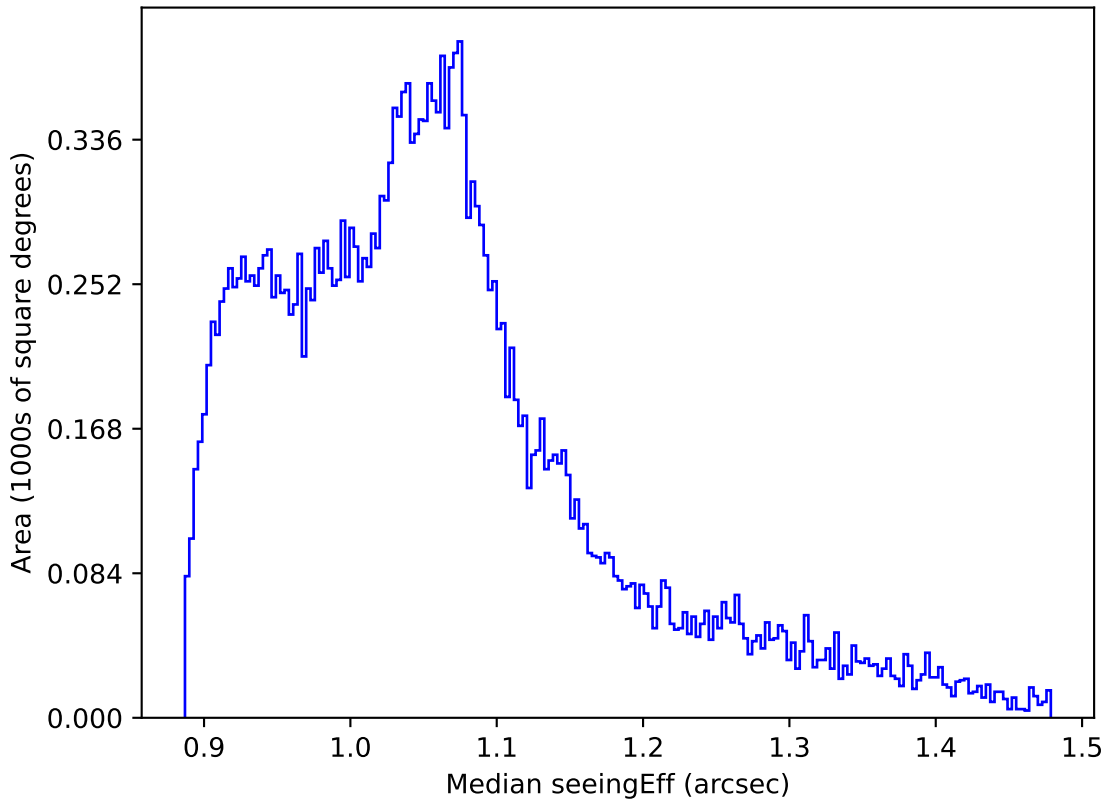
roll_pause_mjdp365_v3.4_10yrs All sky all bands: Median seeingEff
