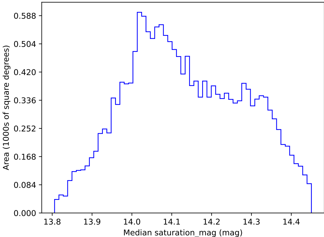
roll_pause_mjdp365_v3.4_10yrs WFD z band: Median saturation_mag
