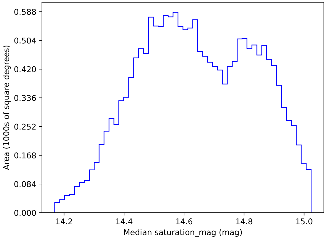
roll_pause_mjdp365_v3.4_10yrs WFD r band: Median saturation_mag
