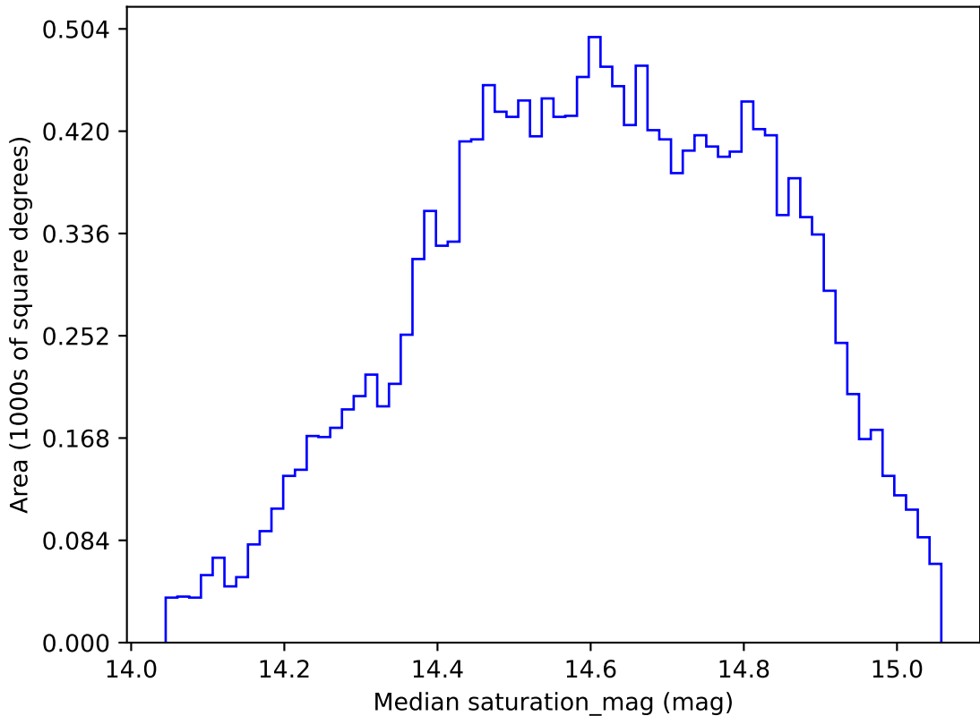
roll_pause_mjdp365_v3.4_10yrs WFD g band: Median saturation_mag
