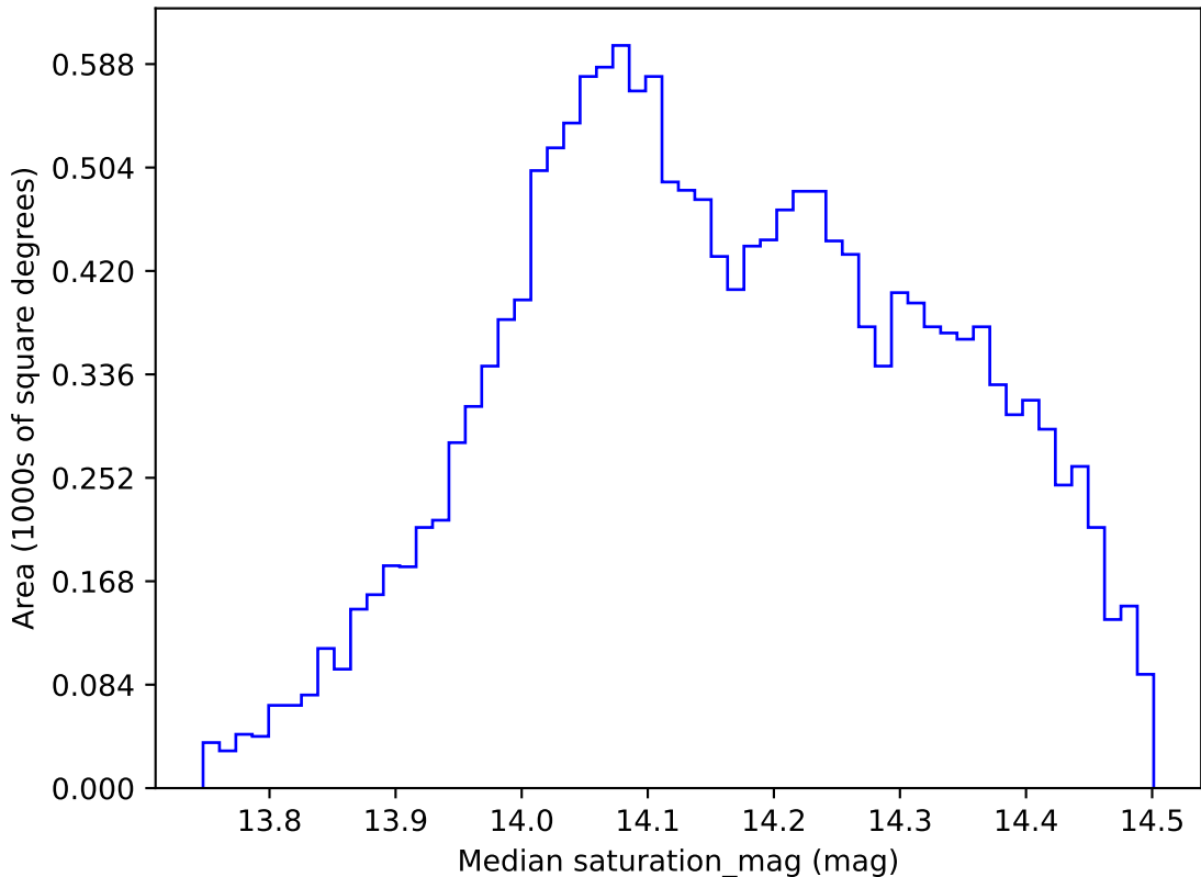
roll_pause_mjdp365_v3.4_10yrs WFD all bands: Median saturation_mag
