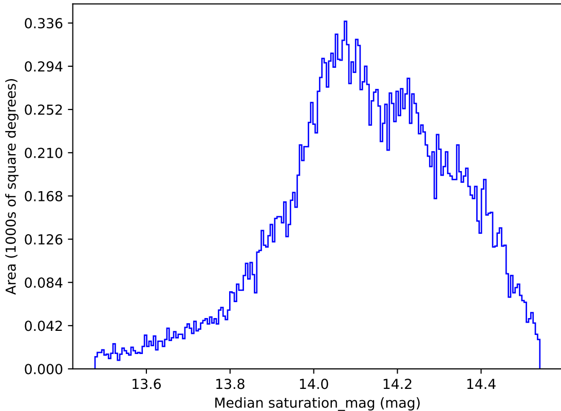
roll_pause_mjdp365_v3.4_10yrs All sky all bands: Median saturation_mag
