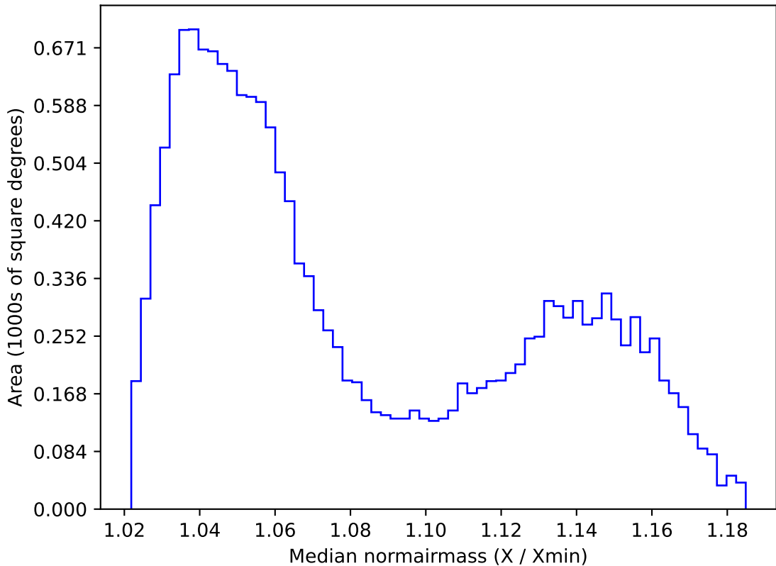
roll_pause_mjdp365_v3.4_10yrs WFD z band: Median normairmass
