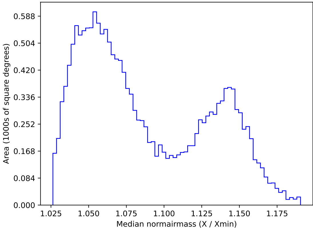
roll_pause_mjdp365_v3.4_10yrs WFD y band: Median normairmass
