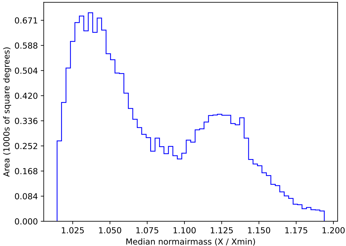
roll_pause_mjdp365_v3.4_10yrs WFD u band: Median normairmass
