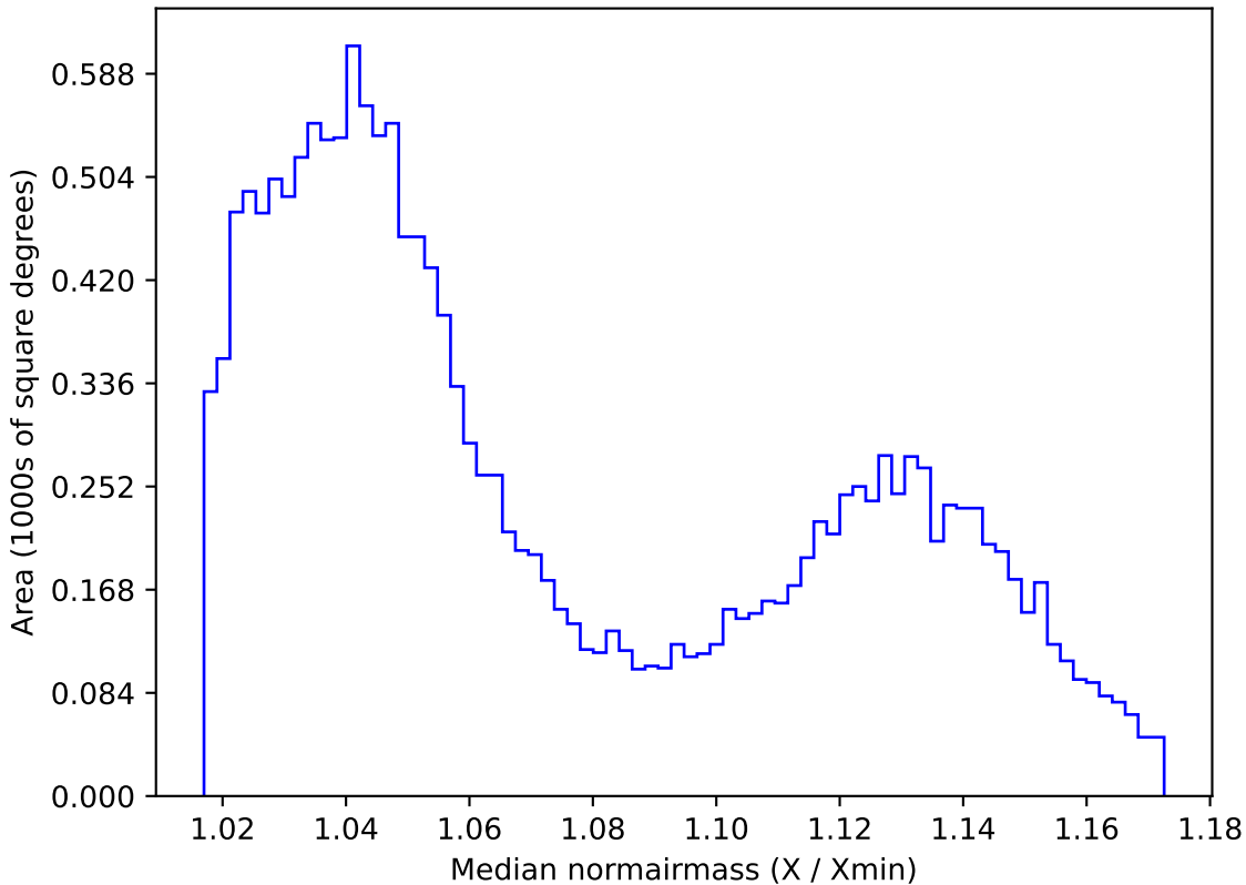
roll_pause_mjdp365_v3.4_10yrs WFD r band: Median normairmass
