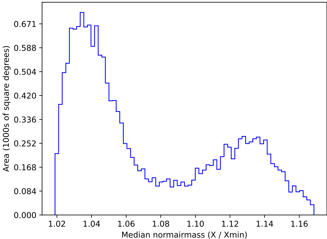
roll_pause_mjdp365_v3.4_10yrs WFD i band: Median normairmass
