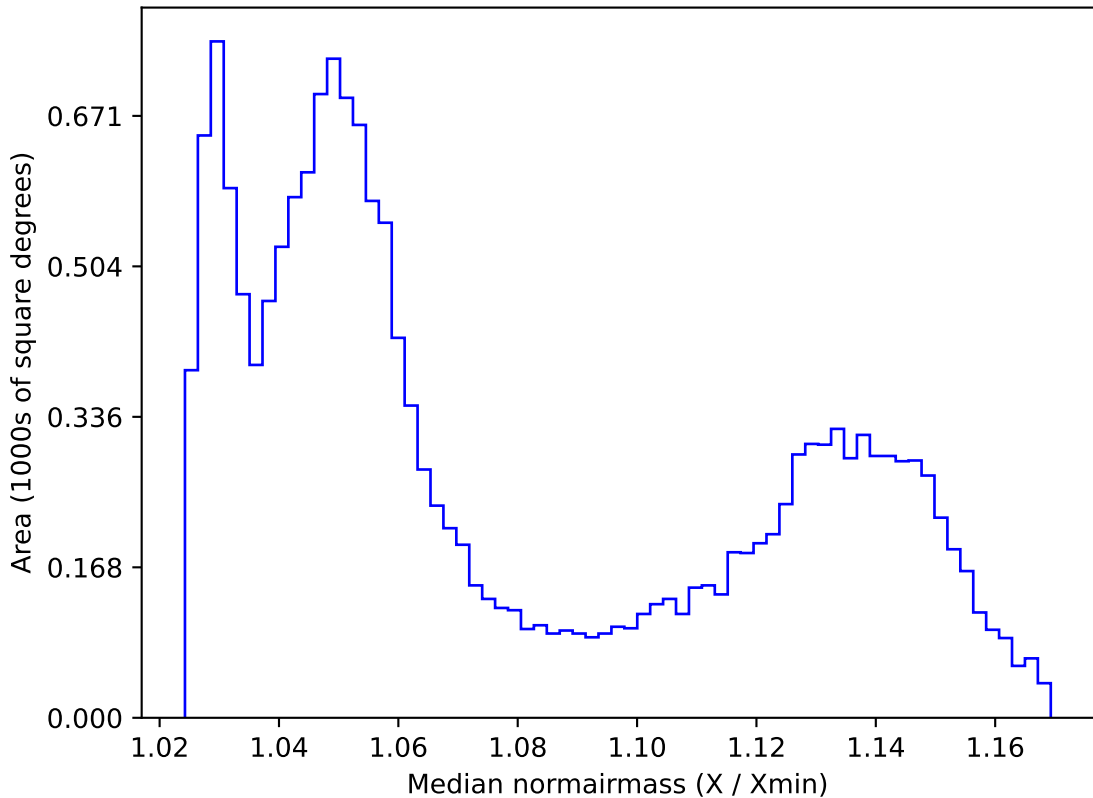
roll_pause_mjdp365_v3.4_10yrs WFD all bands: Median normairmass
