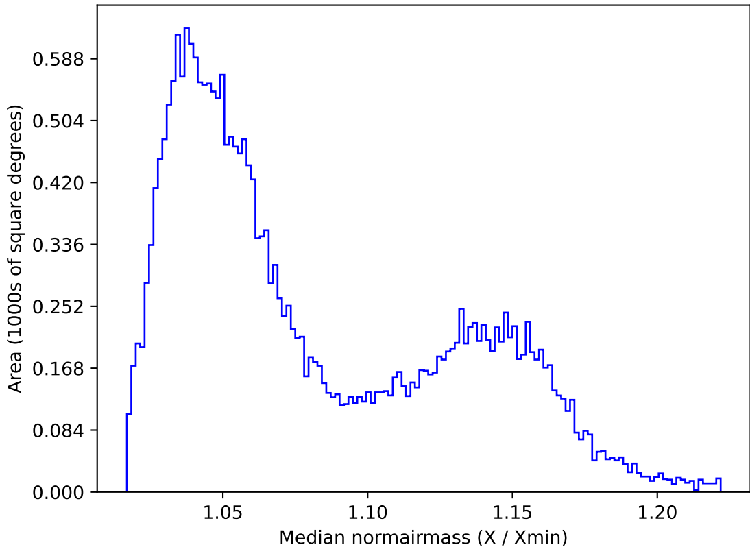
roll_pause_mjdp365_v3.4_10yrs All sky z band: Median normairmass
