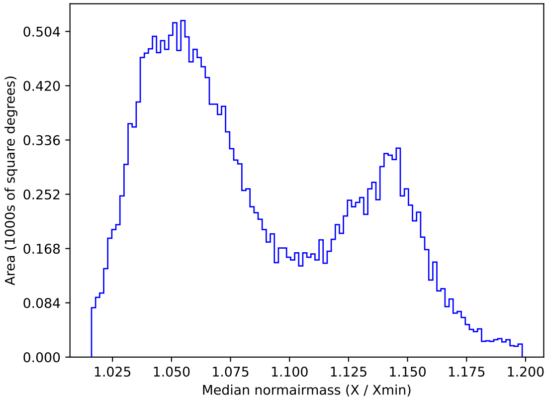
roll_pause_mjdp365_v3.4_10yrs All sky y band: Median normairmass
