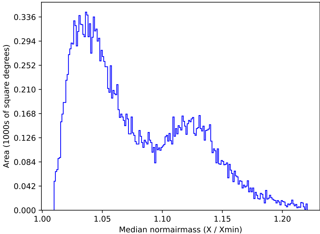
roll_pause_mjdp365_v3.4_10yrs All sky u band: Median normairmass
