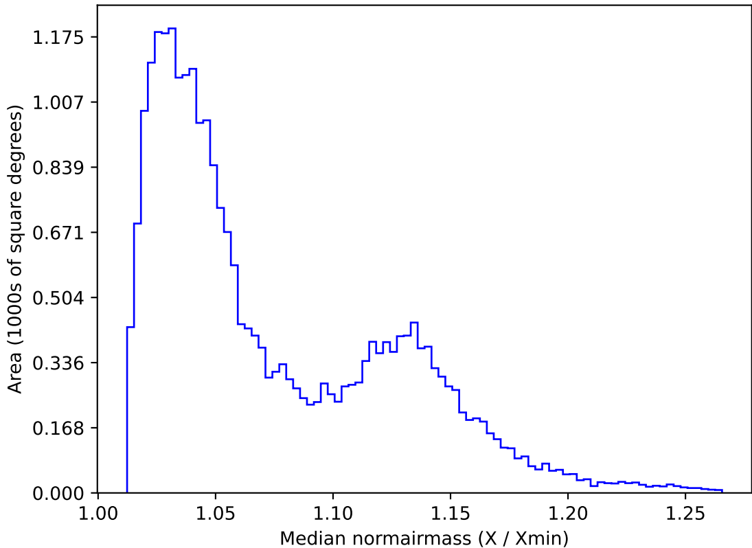
roll_pause_mjdp365_v3.4_10yrs All sky g band: Median normairmass
