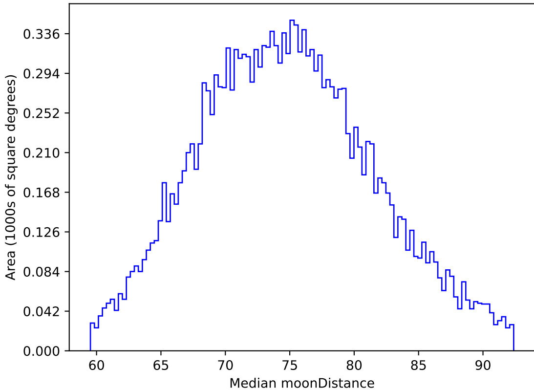
roll_pause_mjdp365_v3.4_10yrs WFD z band: Median moonDistance
