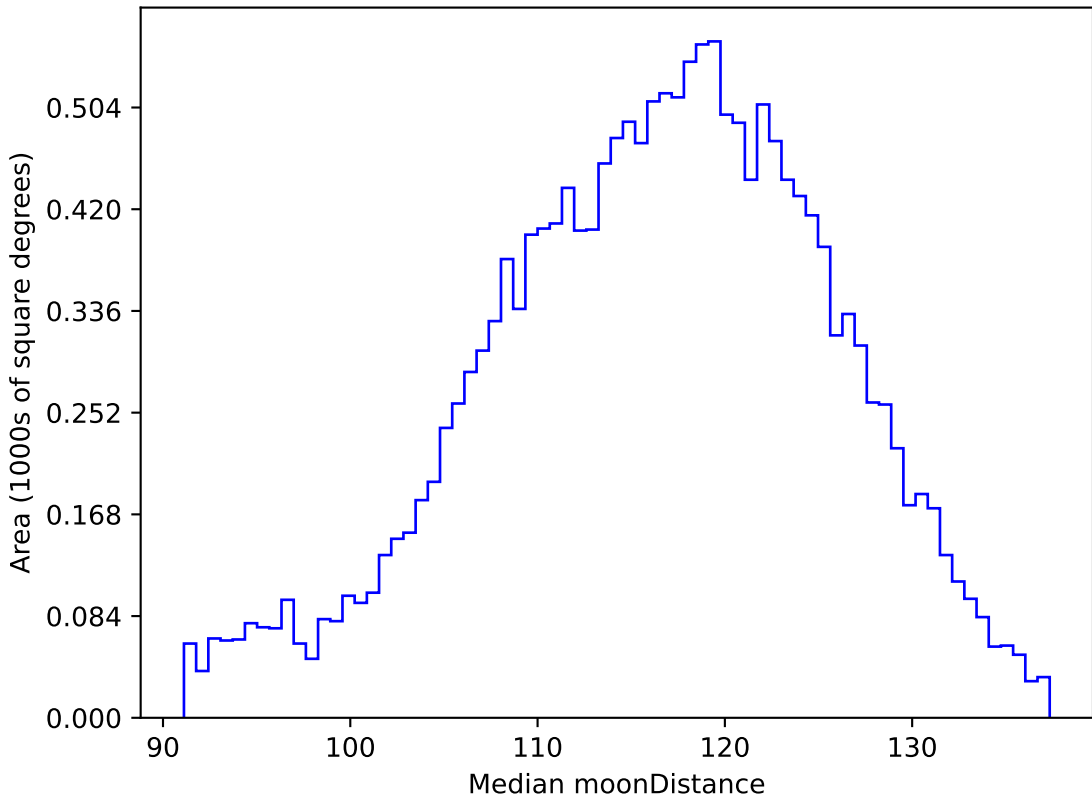
roll_pause_mjdp365_v3.4_10yrs WFD g band: Median moonDistance
