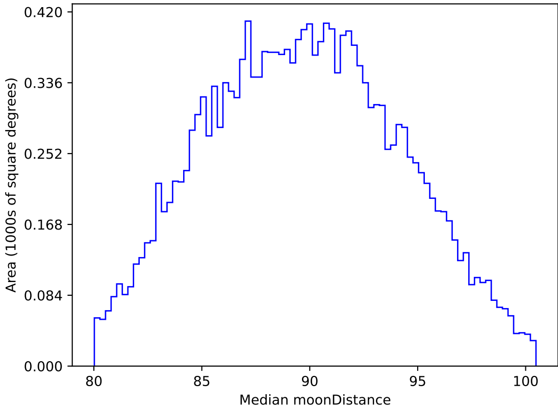
roll_pause_mjdp365_v3.4_10yrs WFD all bands: Median moonDistance
