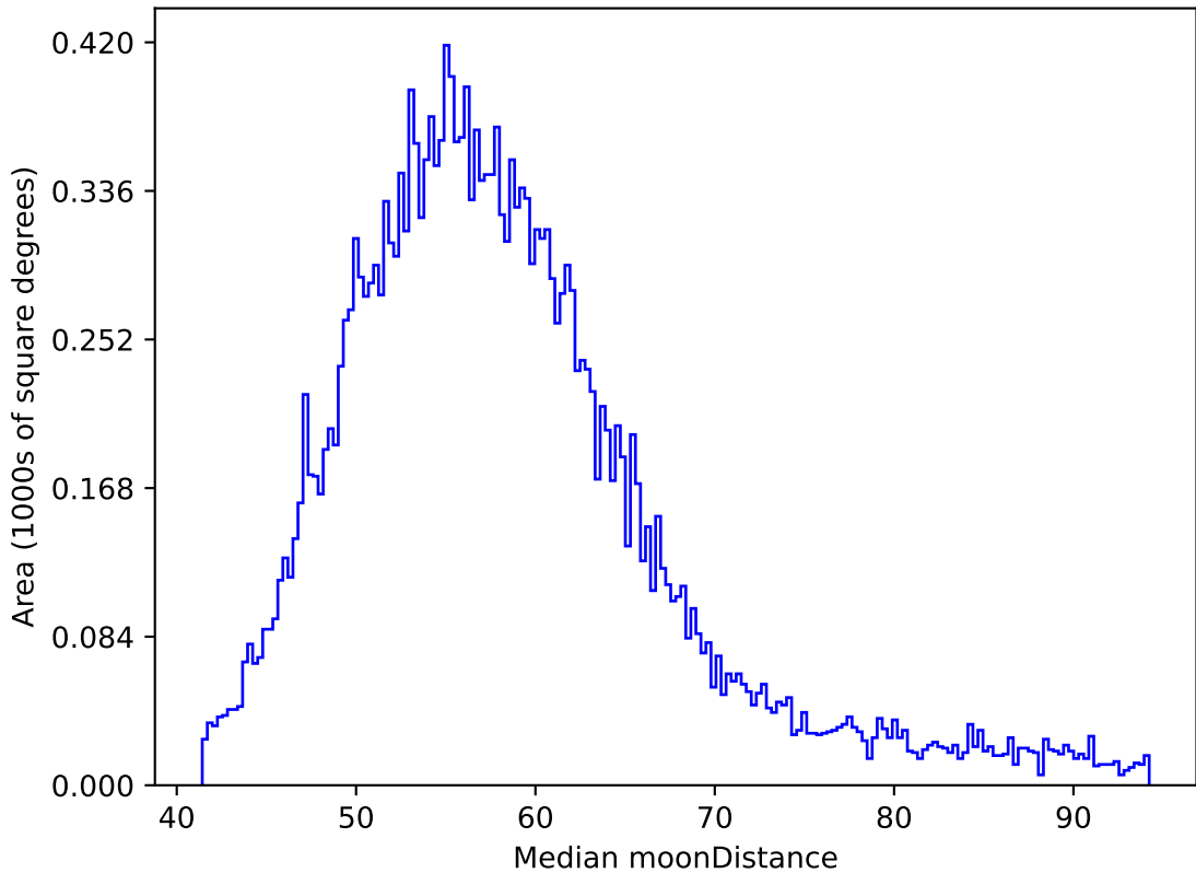
roll_pause_mjdp365_v3.4_10yrs All sky y band: Median moonDistance
