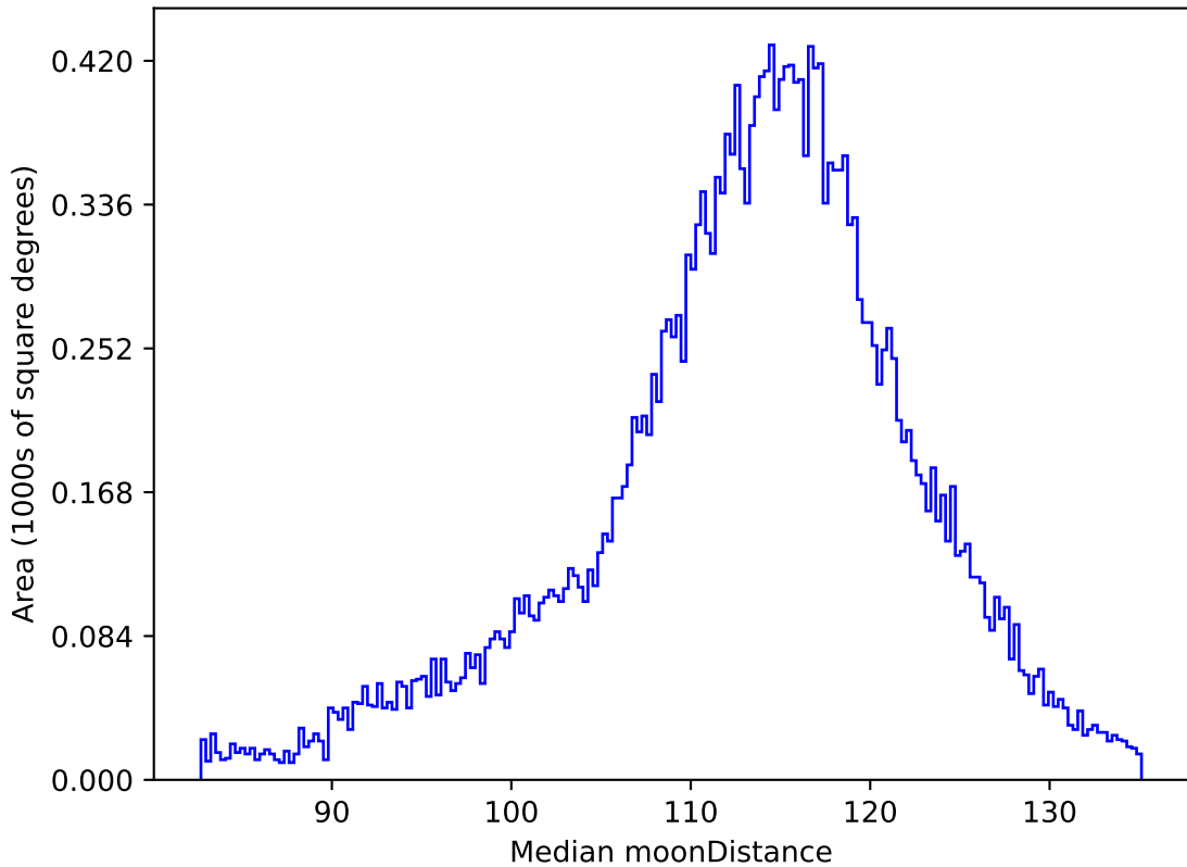
roll_pause_mjdp365_v3.4_10yrs All sky r band: Median moonDistance
