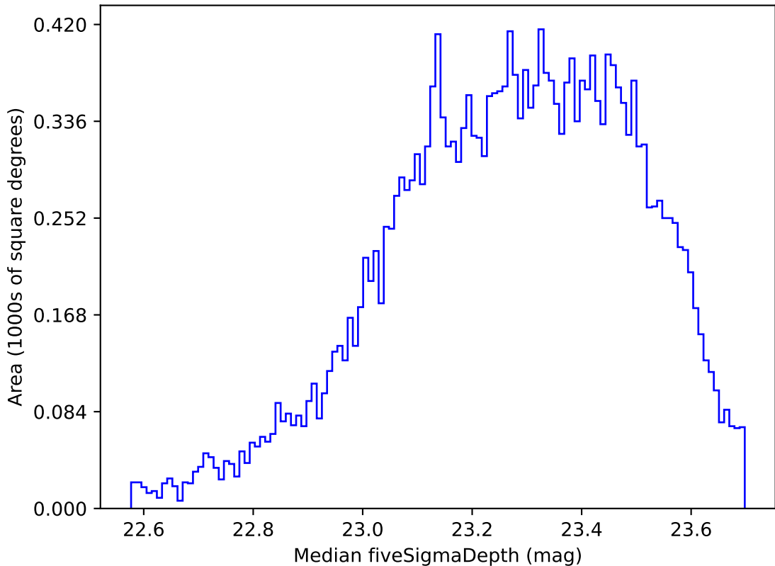
roll_pause_mjdp365_v3.4_10yrs Yr 1 u band: Median fiveSigmaDepth
