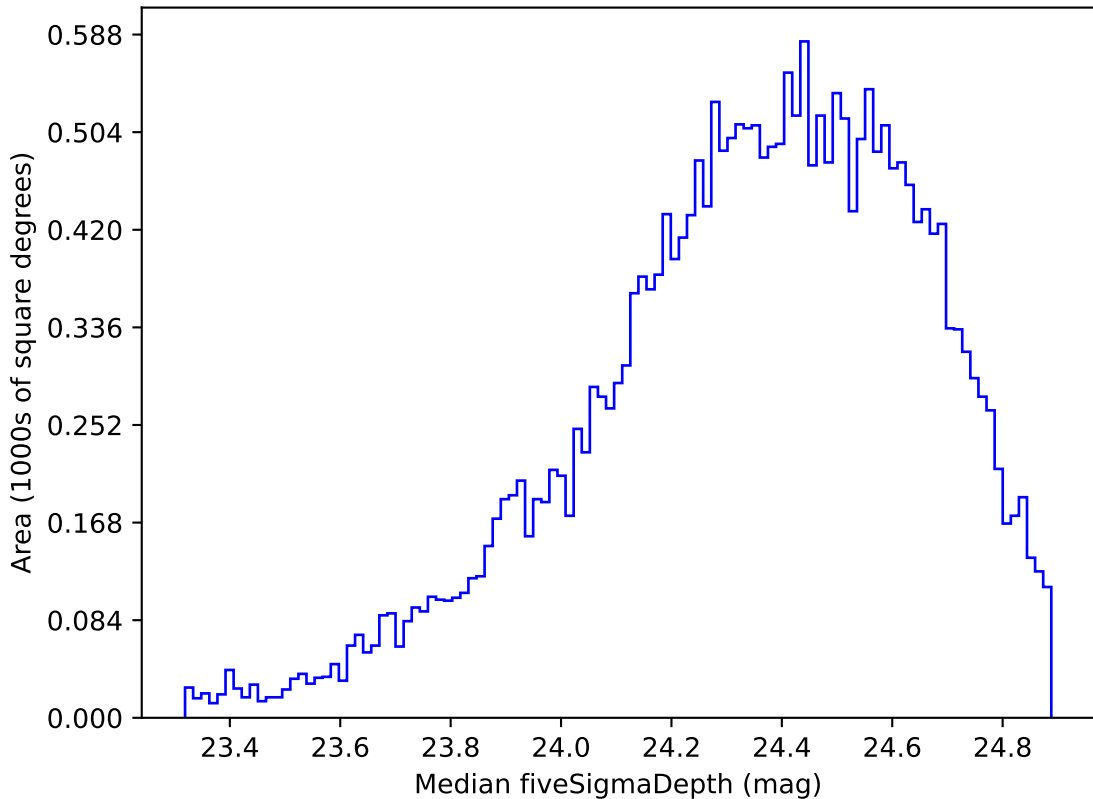
roll_pause_mjdp365_v3.4_10yrs Yr 1 g band: Median fiveSigmaDepth
