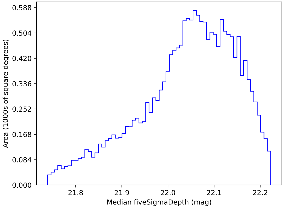
roll_pause_mjdp365_v3.4_10yrs WFD y band: Median fiveSigmaDepth
