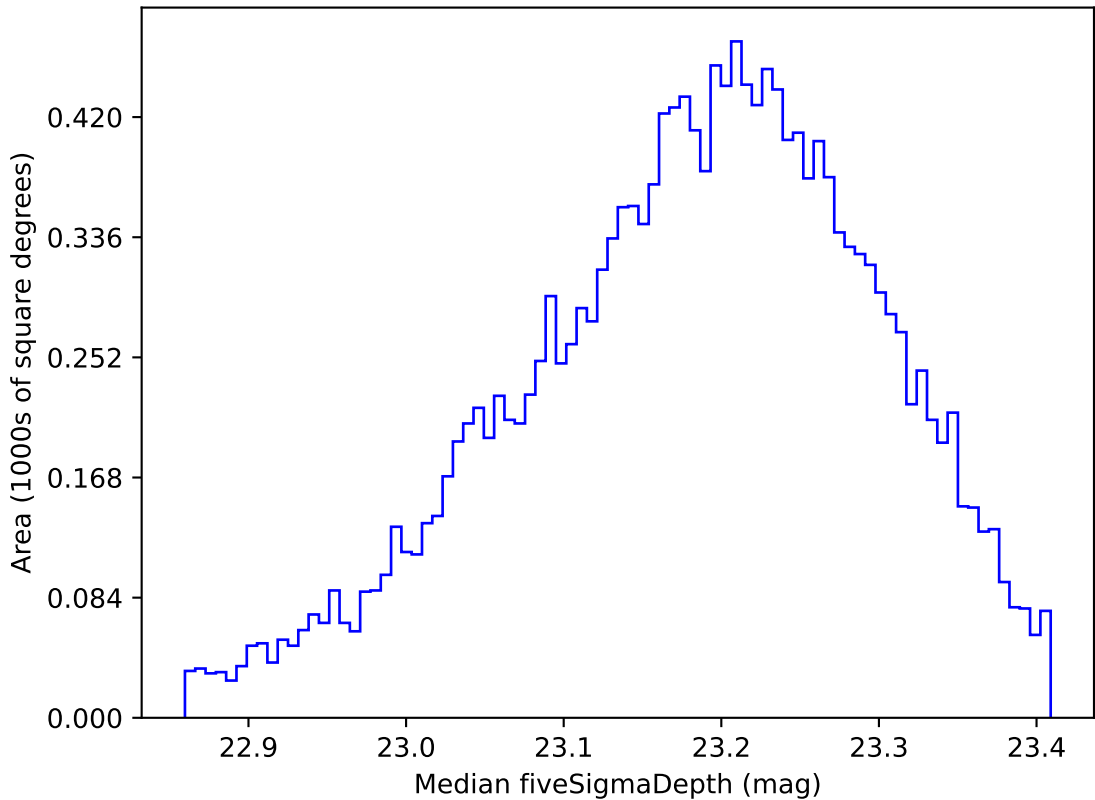
roll_pause_mjdp365_v3.4_10yrs WFD u band: Median fiveSigmaDepth
